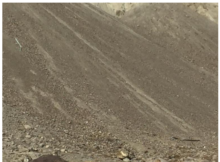
Figure 4: Toppling of boulders, cobbles, pebbles and gravels in the Project area
